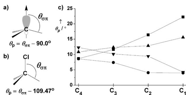
Figure 2. Pyramidalization angles ( \theta_p ) for a) sp^2 and b) sp^3 carbon atoms in chlorofullerenes. c) The \theta_p values of the first four carbon atoms in C_{50} , C_{50}Cl_{10} , C_{64} , and C_{64}Cl_4 . ■ C_{64} , ● C_{64}Cl_4 , ▲ C_{50} , ▼ C_{50}Cl_{10} . The carbon labels are defined in Figure 1.
